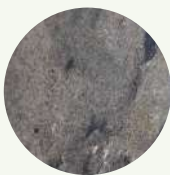
Astrea
